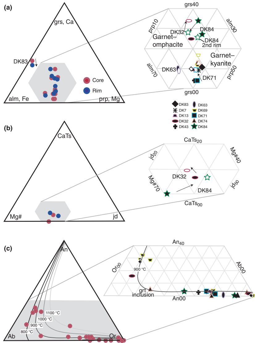
Fig. 3. (a) Grossular–almadine–pyrope compositions of garnet. Arrows show core to rim zoning; (b) Ca–Tschermak, Mg-number and acmite + jadeite components of clinopyroxene; and (c) albite–anorthite–orthoclase compositions of feldspar with solvus isotherms at 17 kbar (Elkins & Grove, 1990). For all samples, the black fill indicates the core composition, whereas the white fill indicates the rim composition.
