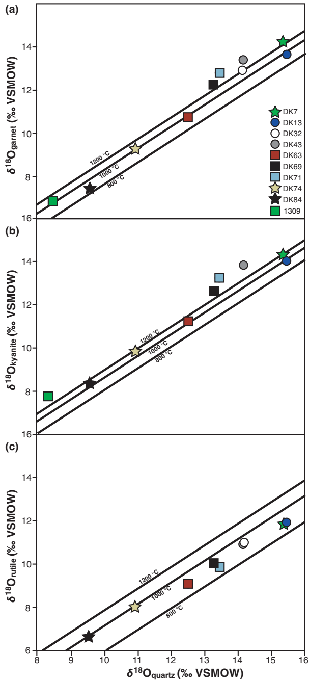
Fig. 4. Values of \delta^{18}\text{O} laser fluorination (a) garnet, (b) kyanite and (c) rutile v. \delta^{18}\text{O} (quartz) with isotherms at 200 °C intervals. Analytical uncertainties are smaller than the symbol size and are thus omitted.
