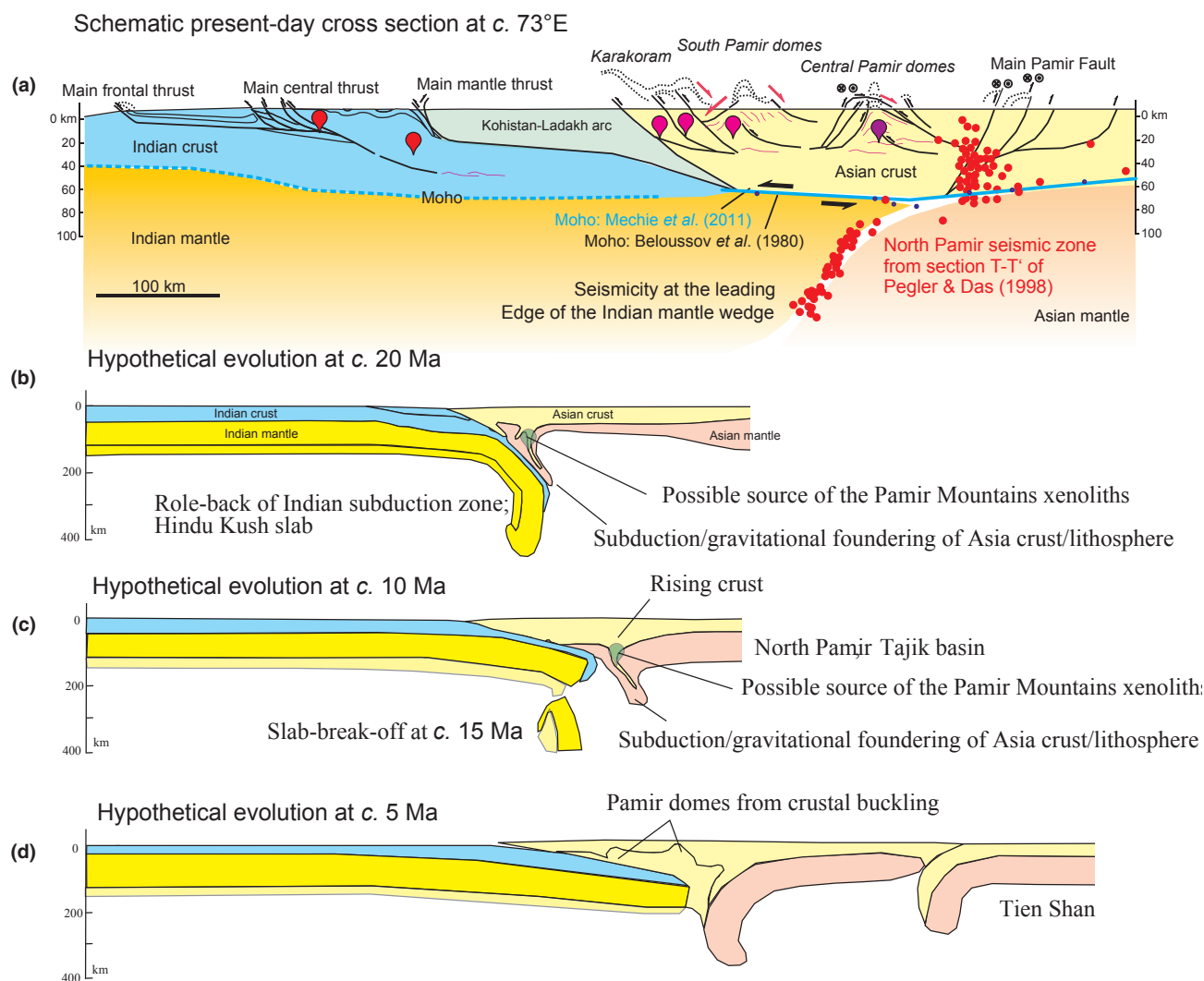
Fig. 12. Schematic N–S cross-section of the India–Asia collision zone with speculative deep extrapolation along \sim 73^\circ\text{E} . The cross sections represent different times in the Pamir Mountains evolution from the (a) present day, (b) c. 20 Ma, (c) c. 10 Ma and (d) c. 5 Ma. The location of the possible source material for the xenoliths is indicated within the cross-section, and figure (a) shows the seismic data used for interpretations of the deep roots of the Pamir Mountains.
